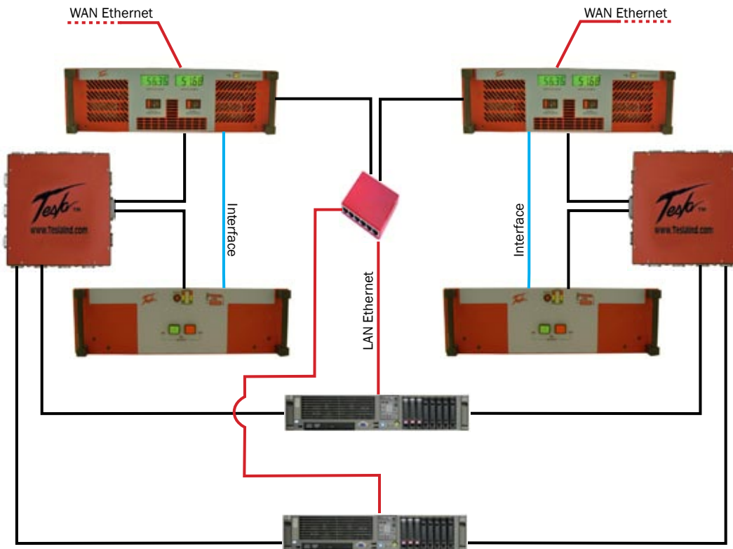
Dual Power Distribution System
